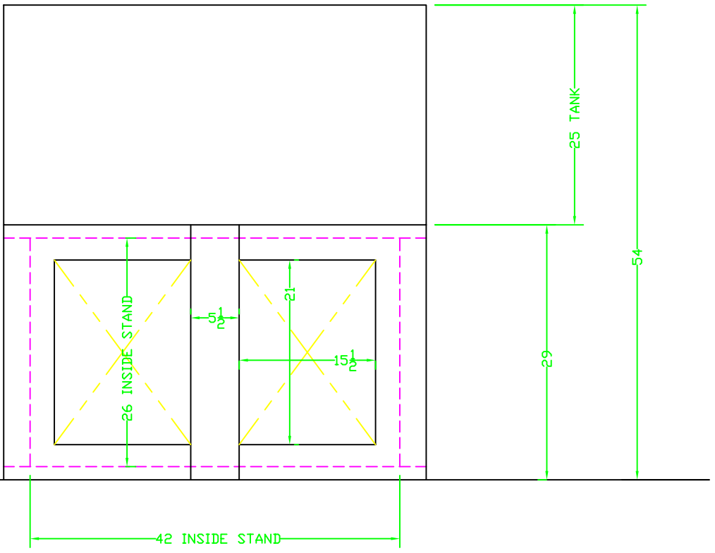
FRONT
